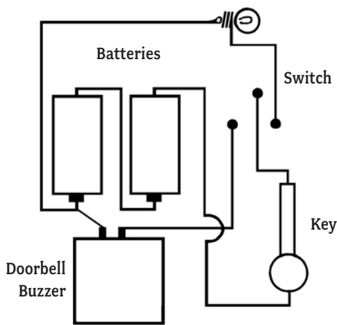
Wiring Diagram
