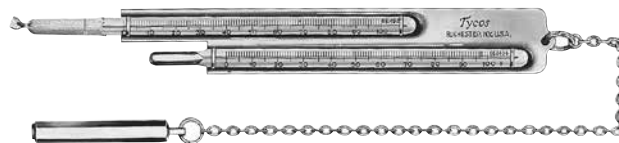
Sling Psychrometer
