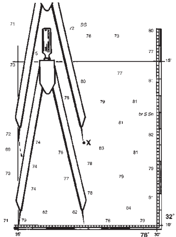
Measuring the longitude of a point on a chart. The longitude is 78°32.7' West.
